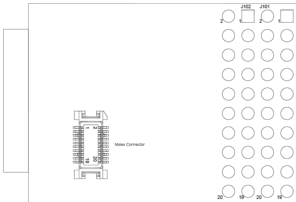
Figure 9: D52Q M6 (Development Module) - Bottom View
