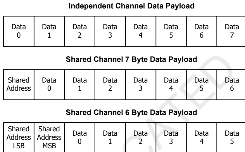
Figure 5-4. Independent and 1 or 2-byte shared channel data payloads.
